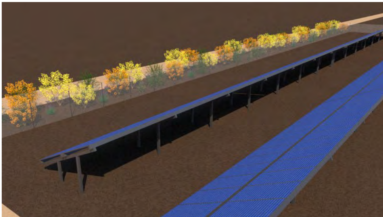
Fig.7 Vista interior de PSFV y Orla Vegetal
